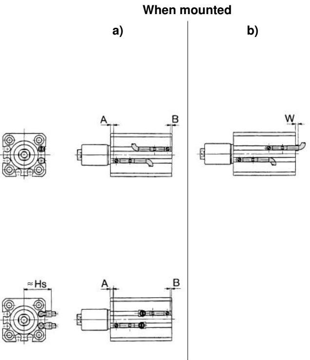
Auto Switch Mounting Height
