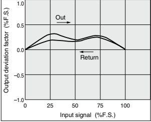
Hysteresis
