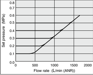
Relief flow characteristics Supply pressure: 0.7 MPa
