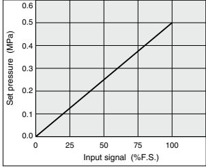
Linearity
