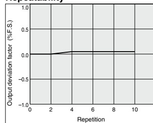
Repeatability
