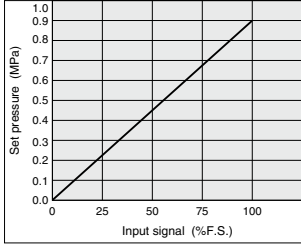
Linearity
