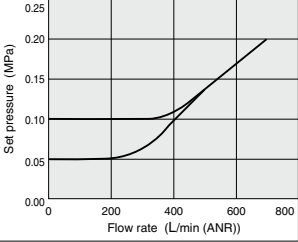
Relief flow characteristics Supply pressure: 0.2 MPa
