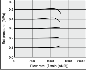
Flow characteristics Supply pressure: 0.7 MPa
