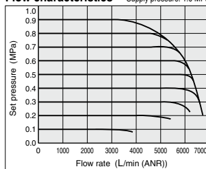
Flow characteristics Supply pressure: 1.0 MPa
