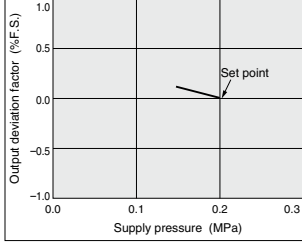
Pressure characteristics Set pressure: 0.05 MPa
