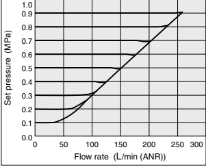
Relief flow characteristics Supply pressure: 1.0 MPa
