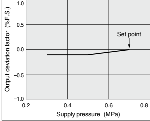
Pressure characteristics Set pressure: 0.2 MPa
