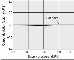
Pressure characteristics Set pressure: 0.4 MPa
