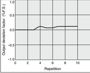
Repeatability
