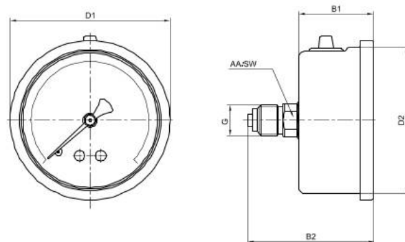
02-Back Connection
