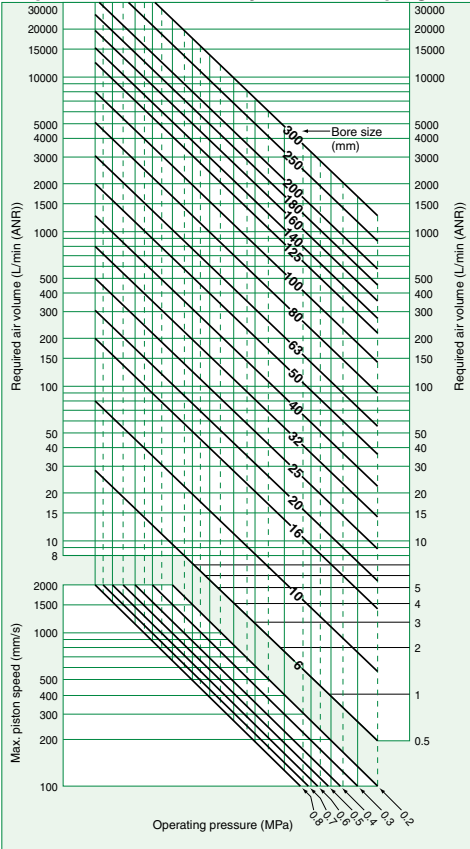
Required Air Volume of Cylinder and Piping
