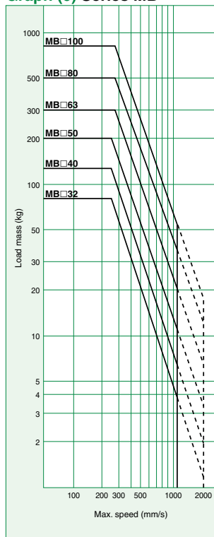
Graph (6) Series MB
