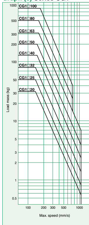
Graph (8) Series CG1
