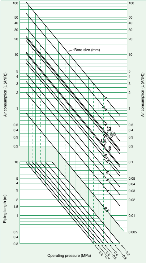
Air Consumption of Tube or Steel Pipe (For one cycle)
