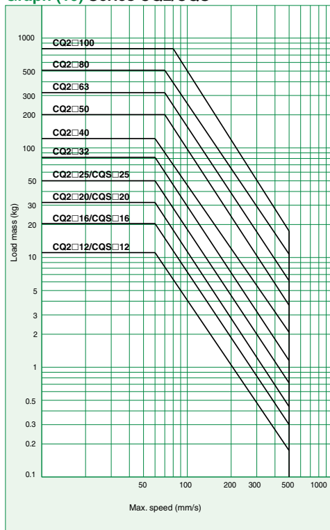
Graph (10) Series CQ2/CQS
