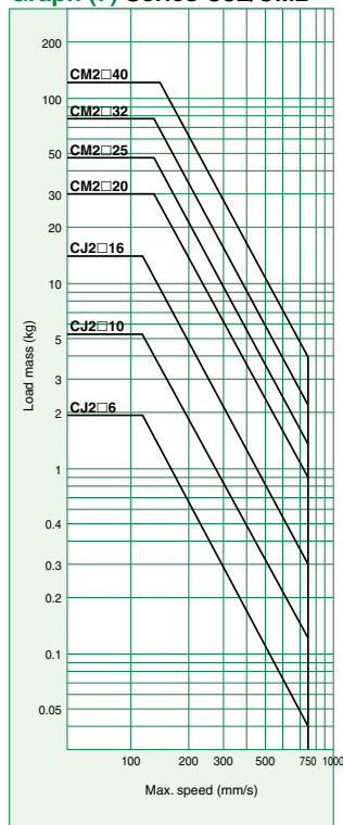
Graph (7) Series CJ2/CM2
