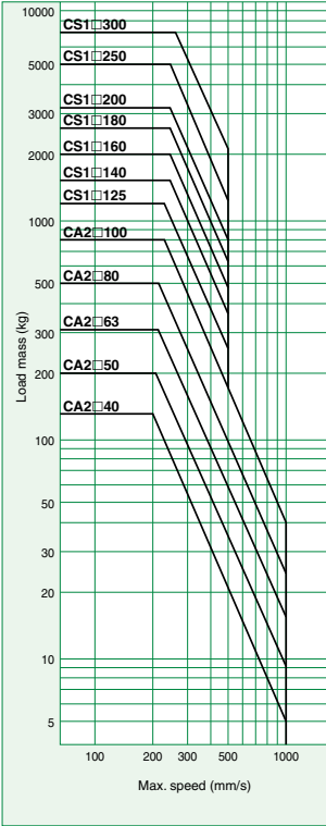
Graph (5) Series CA2/CS1
