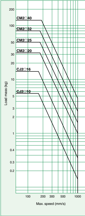
Graph (3) Series CJ2/CM2
