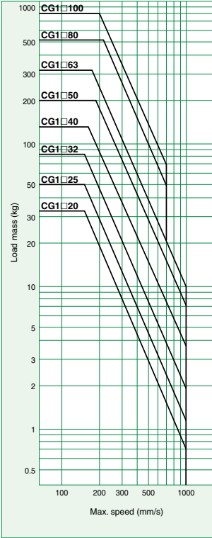
Graph (4) Series CG1
