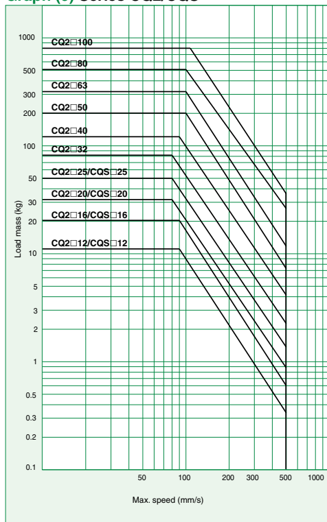
Graph (9) Series CQ2/CQS
