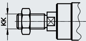
K5 – Custom piston rod thread
