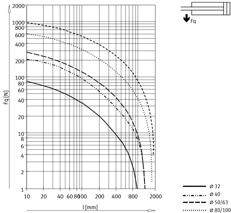
Max. transverse load Fq as a function of stroke length l
